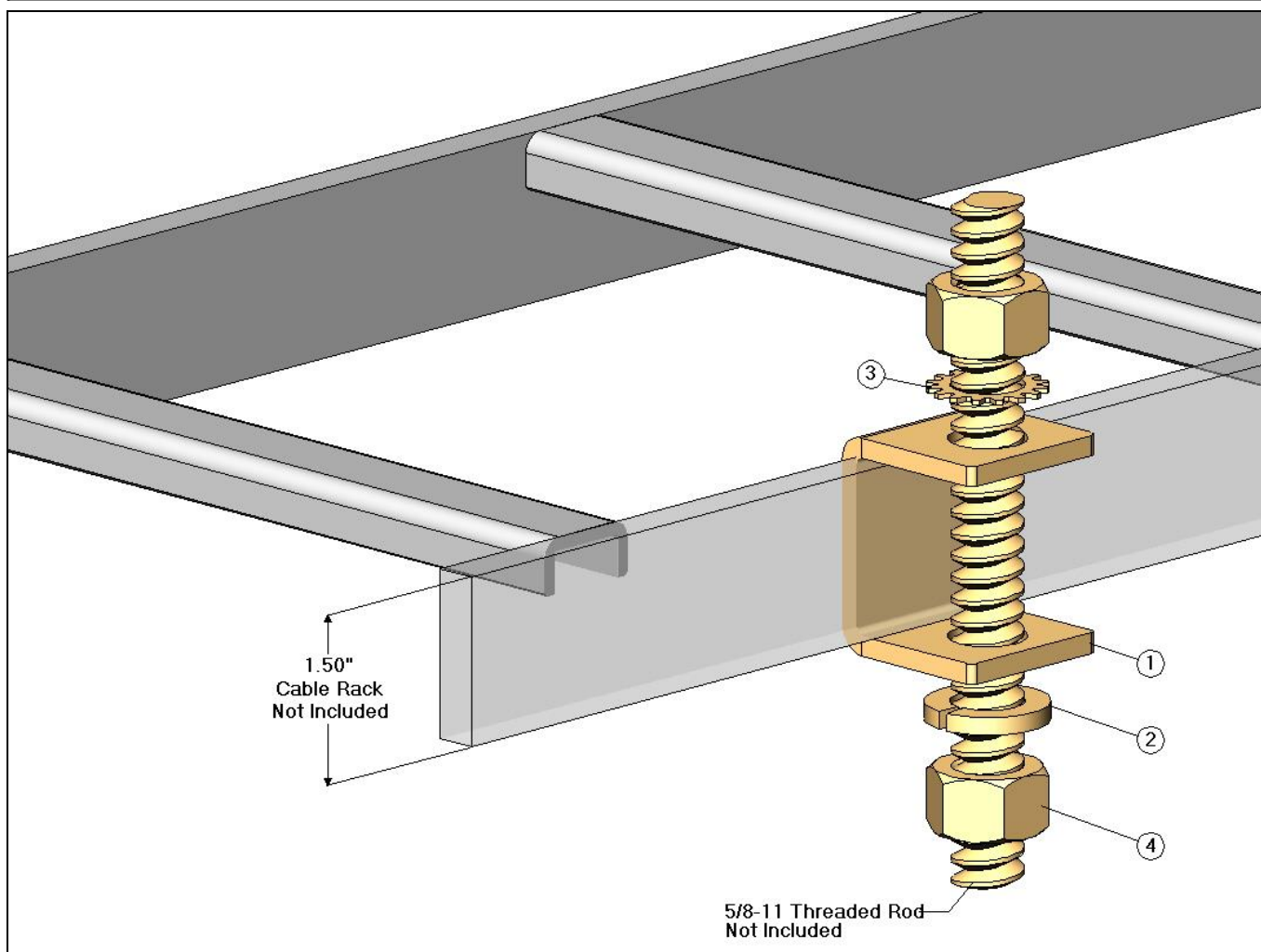
HB1x Series - 1.50" Cable Rack Hanger Kit Selection
